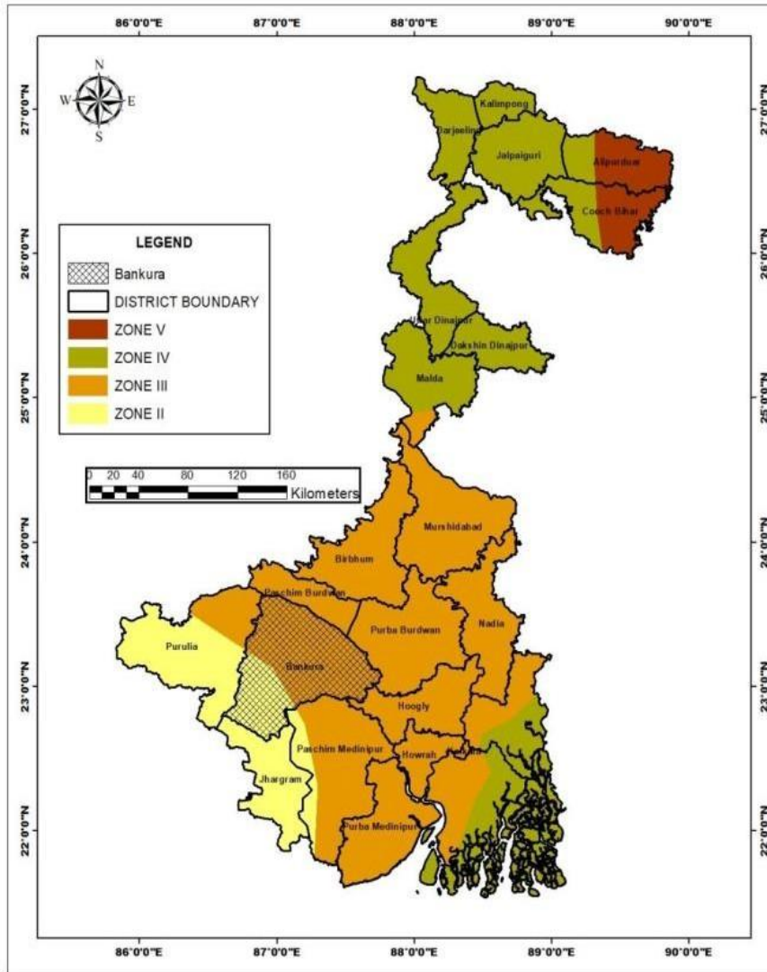
Figure 2.8: Seismic Map of the State of West Bengal (Source: Amateur Seismic Centre (ASC), Pune, 2022)
