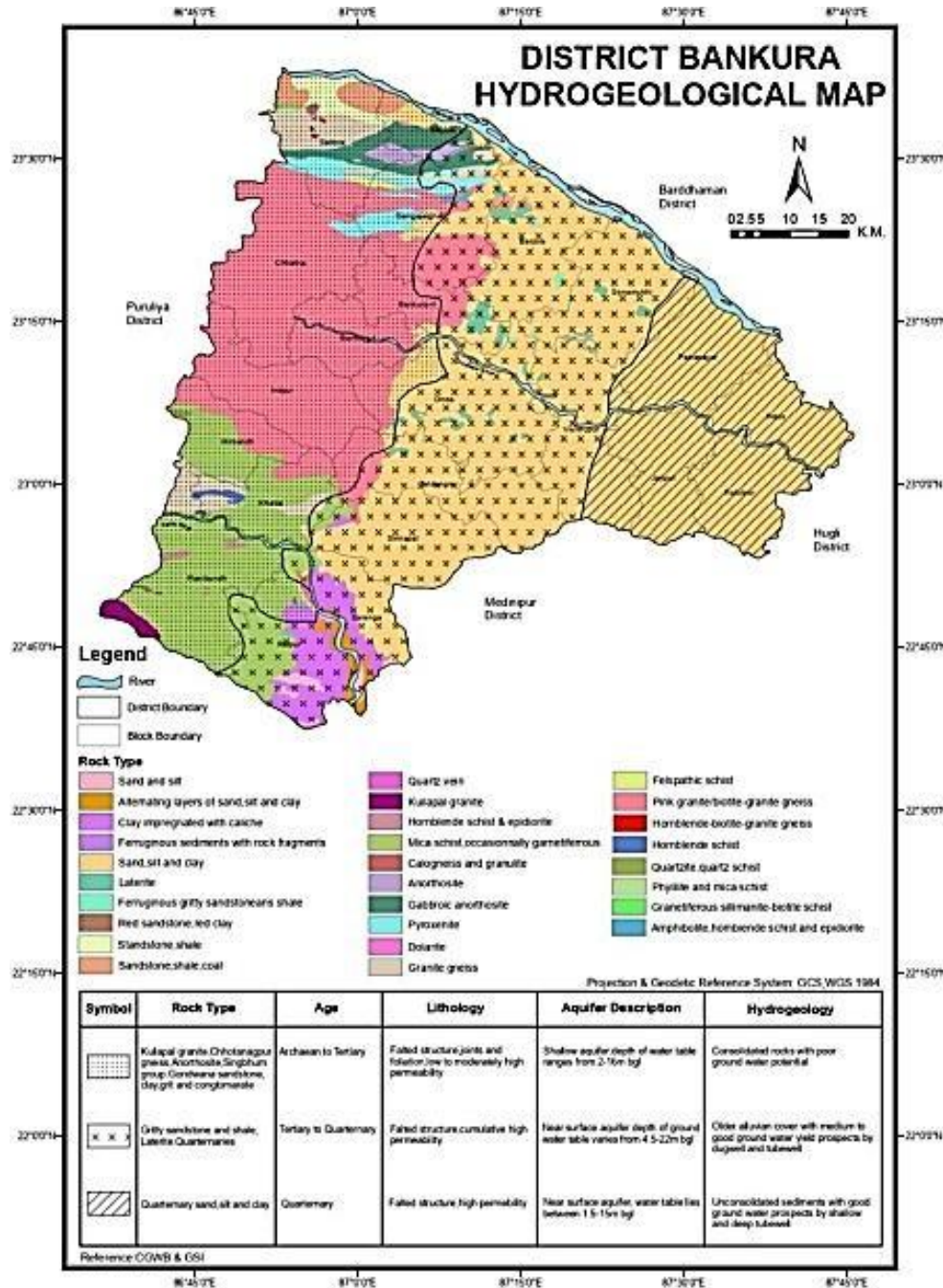
Figure 2.5: Hydrogeological map of the Study area in Bankura District, West Bengal
