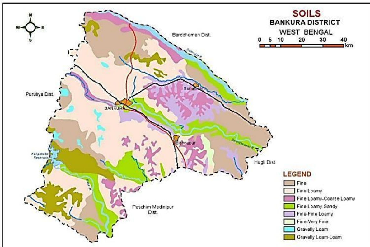
Figure 2.1: Soil Map, Bankura District, West Bengal
