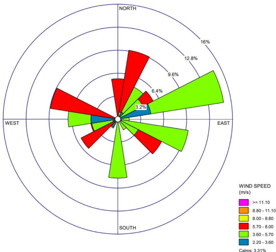
Figure 3-8: Wind rose diagram. Wind Class Frequency Distribution
