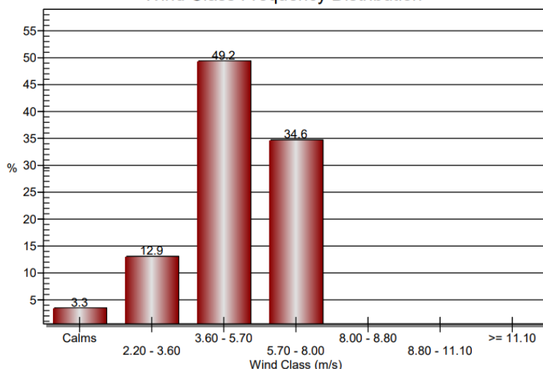
Figure 3-9: Wind Class Frequency Distribution.
